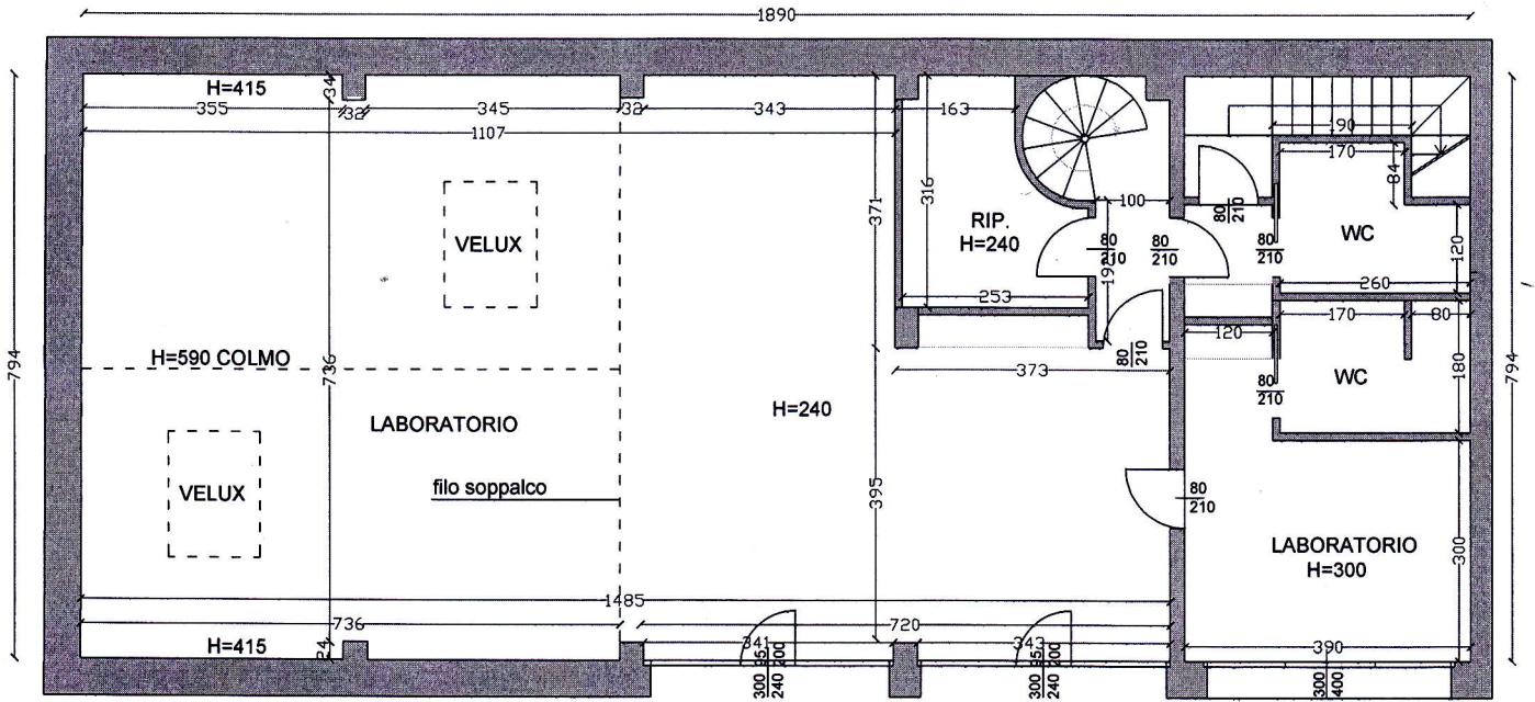
PIANO TERRA mq 150
