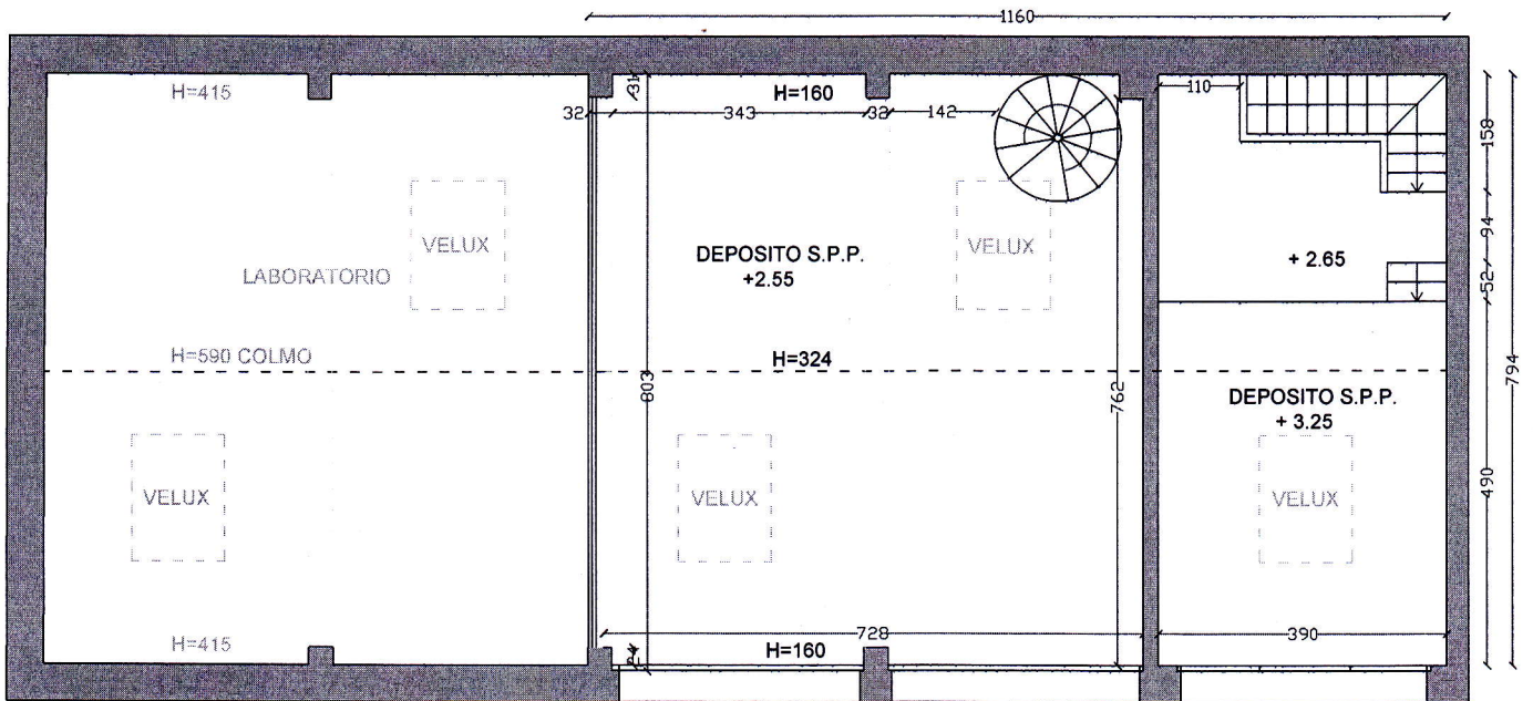
PIANO SOPPALCO S.P.P. mq 90
